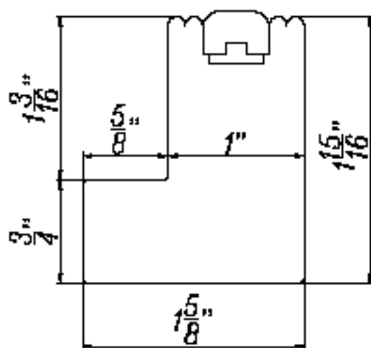
L Frame with Plain Insert
